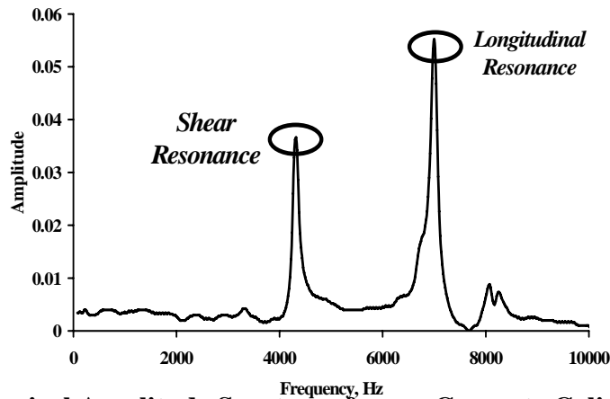
Figure A.16 - Typical Amplitude Spectrum from a Concrete Cylindrical Specimen
