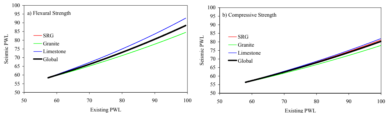
Figure D.7 - Variations in Simulated PWL from Strength Tests and Seismic Tests for All Three Types of Aggregates
