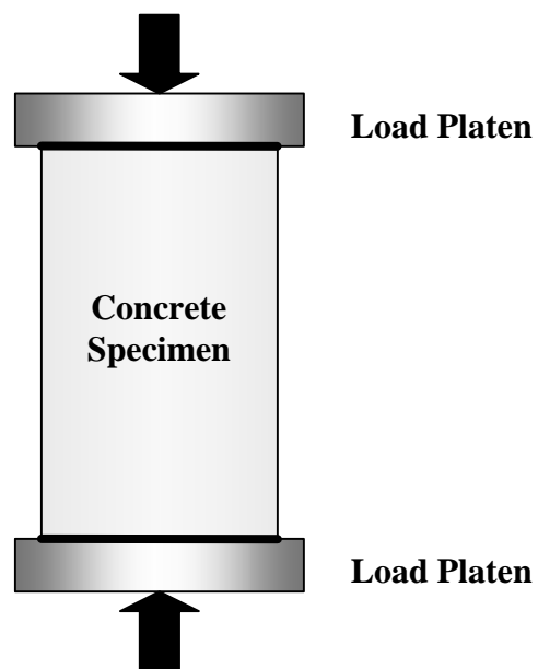
Figure A.6 - Schematic of Compressive Strength Test
